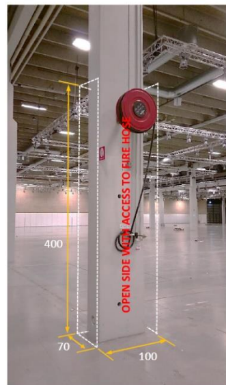
SELF-STANDING BOX TO COVER PILLAR ON 3 SIDES NEXT TO ARCADE C3/C4
